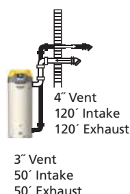
Sealed Direct Vent Sidewall
