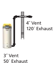
Indoor Conventional Sidewall
