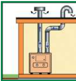
Vertical direct-venting top intake/exhaust
