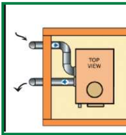
Horizontal sidewall direct-venting rear intake/exhaust
