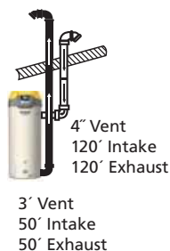
Sealed Direct Vent Vertical
