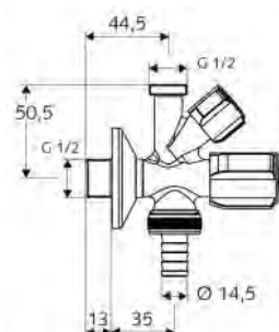
03 569 0699 1/2" x 3/4" combination angle valve
