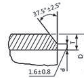
(a)壁厚 ≤ 22 Wall Thickness ≤ 22
