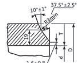
(b)壁厚 > 22 Wall Thickness > 22
