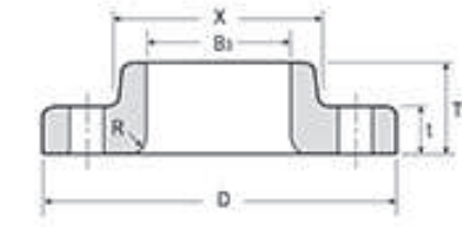
LAP JOINT
