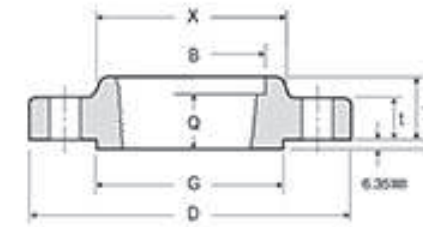
THREADED
