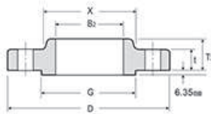
SLIP-ON
