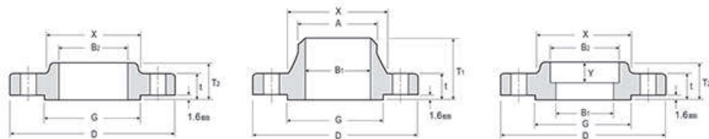
SLIP-ON
