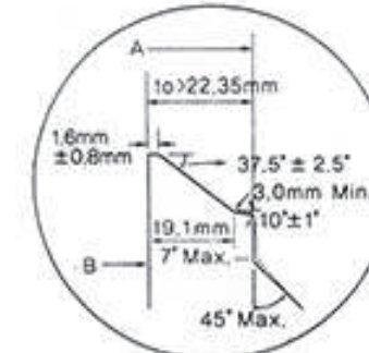
BEVEL FOR WALL THICKNESS(to) GREATER THAN 0.88 IN.(22.35mm)
