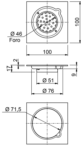
103F/51 Attacco - Connection Ø 51mm
