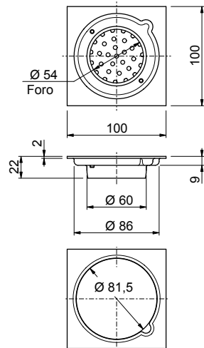
103F Attacco - Connection Ø 60mm
