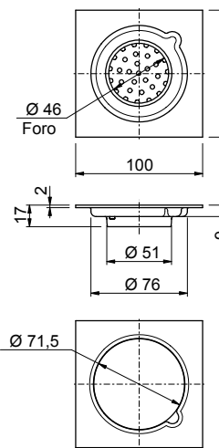
103SF/51 Attacco - Connection Ø 51mm
