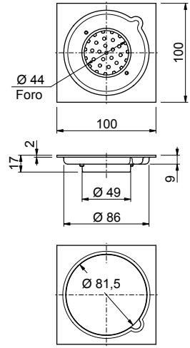
103F/49 Attacco - Connection Ø 49mm
