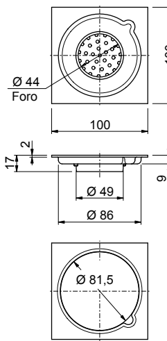
103SF/49 Attacco - Connection Ø 49mm
