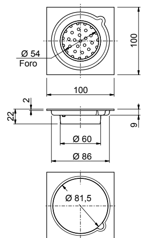
103SF Attacco - Connection Ø 60mm
