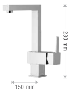
506/QN € 200,00 Miscelatore monocomando lavello bocca girevole. Single lever sink mixer with swivel spout.
