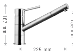
508/HR HERMÉS Miscelatore monocomando lavello bocca girevole. Single-lever sink mixer with swivel spout.
