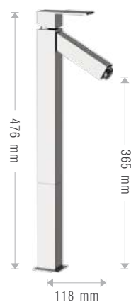
38L/TW € 505,00 Miscelatore lavabo alto XL, con luce led, senza scarico. High wash basin mixer XL version, with led light without waste.
