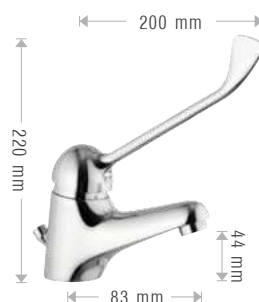
389/E9 € 75,00 Miscelatore monocomando lavabo con leva clinica. Single lever basin mixer with clinical lever.
